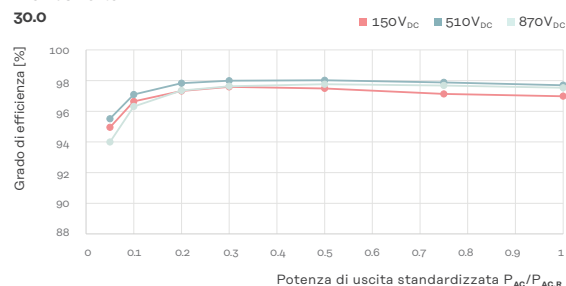
Fronius Verto 30.0
