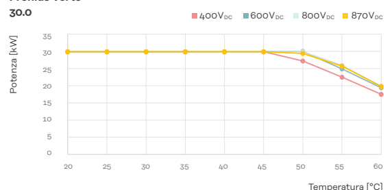
Fronius Verto 30.0
